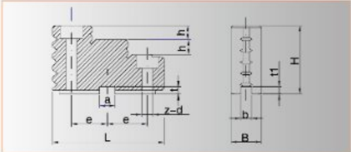
C型分离爪 Two-piece Jaws for Form C
