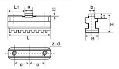
C型分离爪上爪 Two-piece top jaws for form C
