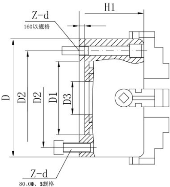
K72——四爪单动卡盘(美标) K72 Four-jaw independent chucks (American-standard)
