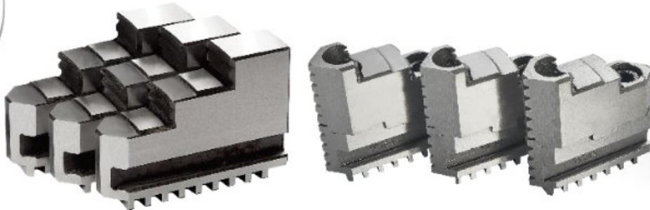
整体爪 One-piece jaw
