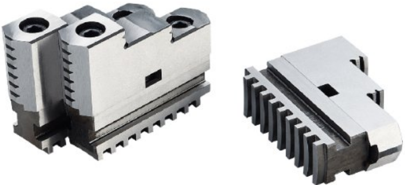
C型分离爪 Two-piece jaws for Form C
