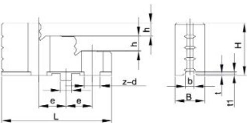
A型、D型分离爪上爪 Two-piece top jaws for form A,D
