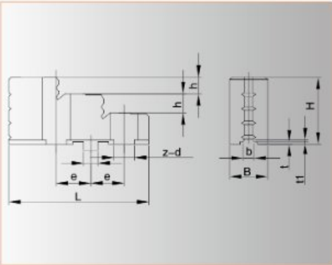
A型、D型分离爪 Two-Piece Jaws for Form A, D
