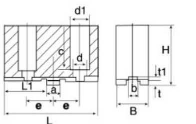
软顶爪 (A型) Soft top jaws (type A)
