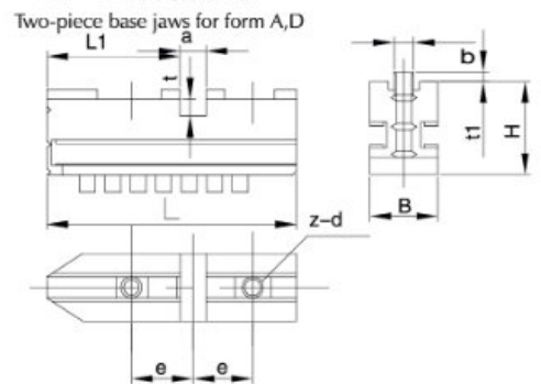
A型、D型分离爪基爪 Two-piece base jaws for form A,D
