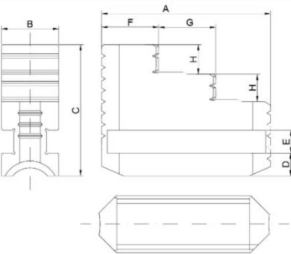
K72卡爪 K72 Jaws
