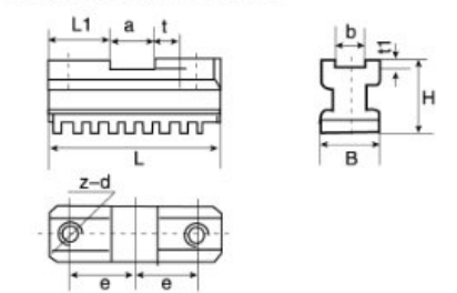
C型分离爪基爪 Two-piece base jaws for form C
