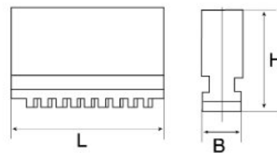
整体软爪 One-piece soft jaws
