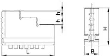
整体爪 One-piece Jaws
