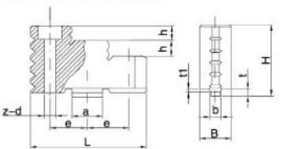
C型分离爪上爪 Two-piece top jaws for form C
