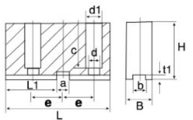
软顶爪 (C型) Soft top jaws (type C)
