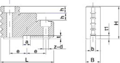
C型分离爪基爪 Two-piece base jaws for form C
